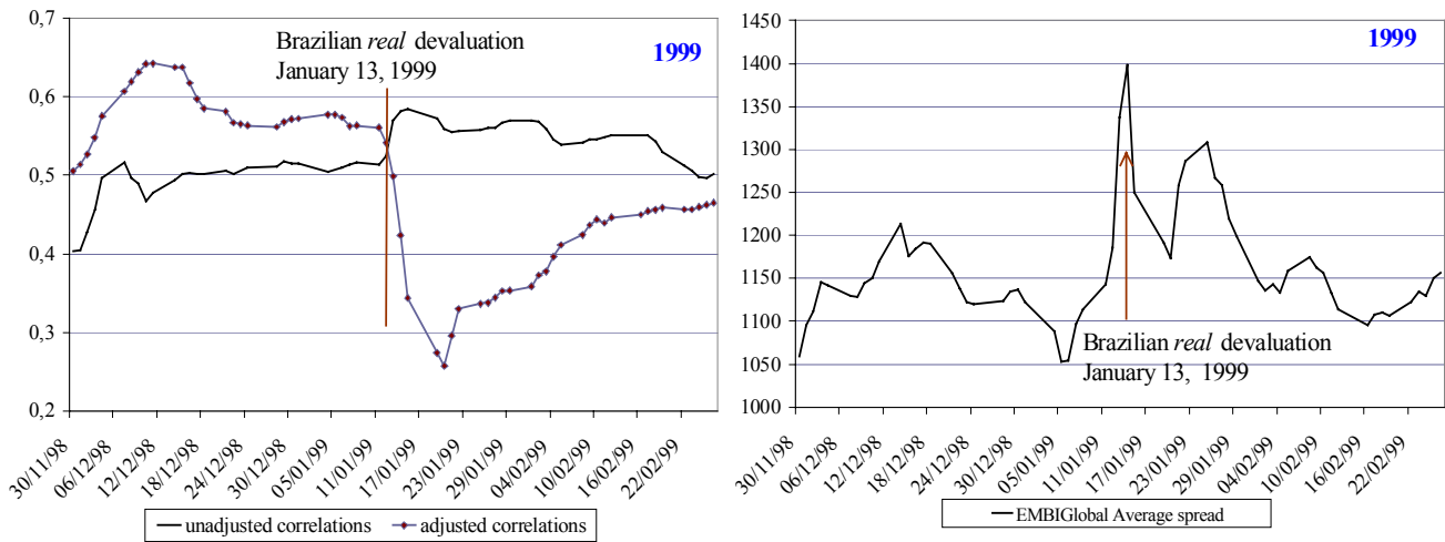
Figures 10a-b: Evolution of correlations and spreads during the Brazilian real devaluation
