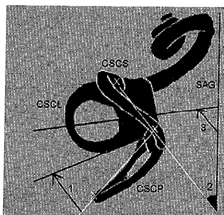
Figure 3 Angular measurements between semi-circular canals ; cscl: lateral semi circular canal, cscp: posterior semi circular canal, cscs: superior semi circular canal, ax: great axis of the lateral semi circular canal, sag: sagittal plane, X: cross section of the posterior and superior canals in the lateral canal plan
