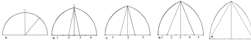
Figure 3: Various arch kinds; a) circular arch : the centre is on the axis. b) Two quarters and a half arch: inherited from the Clunisiens who imported it from the East. The centre of the arches is at 5/8 of the arch basis. c) Three point arch: centre at 2/3 . d) Five point arch: centre at 4/5 . e) Common arch: any point as centre.
