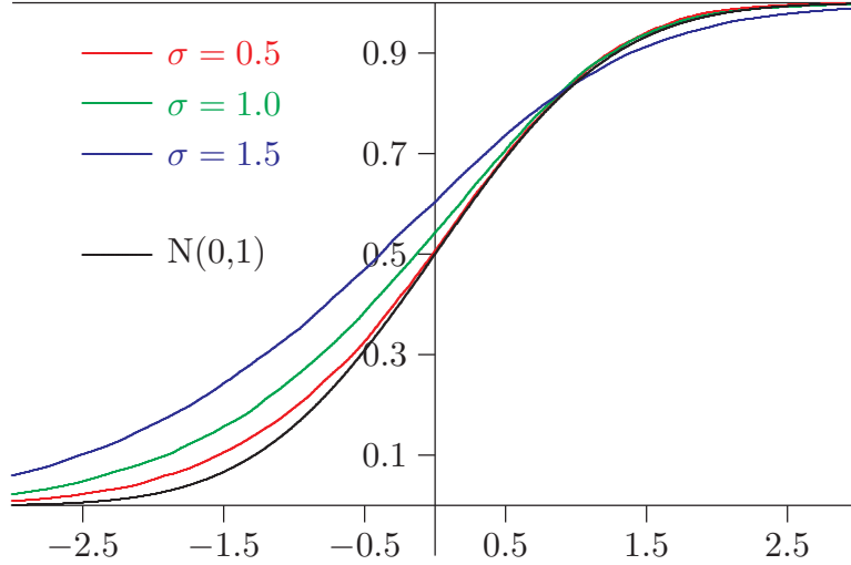
Figure 4. Distribution of \tau for the lognormal distribution
