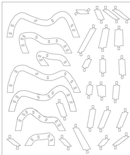
Figure 7 Final setting of pieces ready to cut
