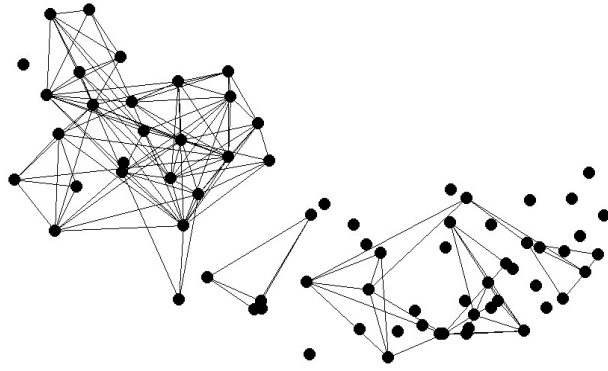
Figure 8 Reciprocal over-attractions, second period
