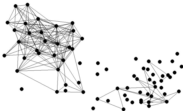
Figure 10 Reciprocal over-attractions, third period
