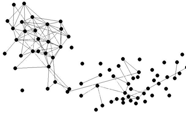
Figure 9 Triads of type 15 or 16, second period
