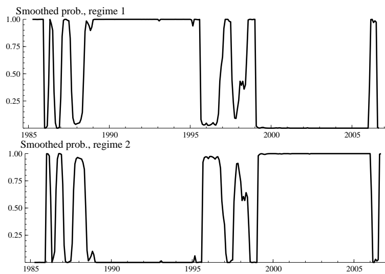
Figure 4. Regime probabilities for MS-SFAVAR
