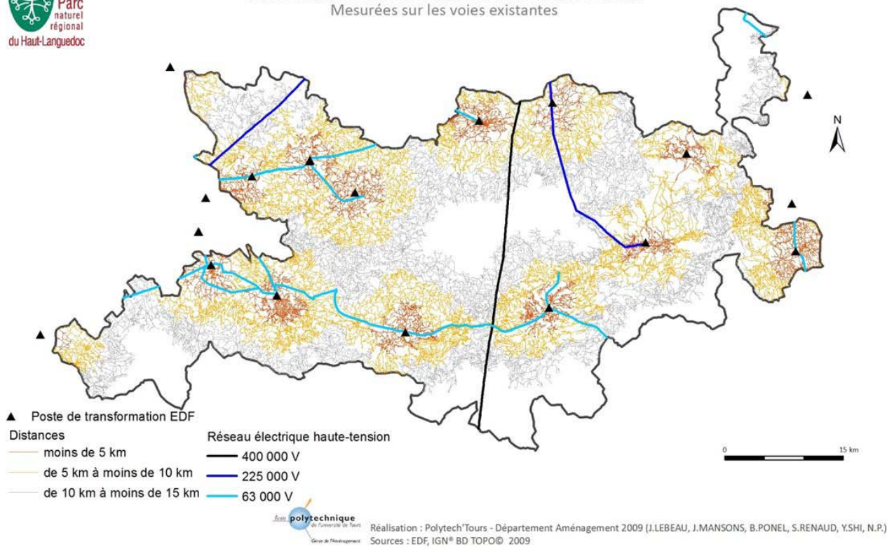
Figure 9 – Infrastructures et distances aux postes sources
