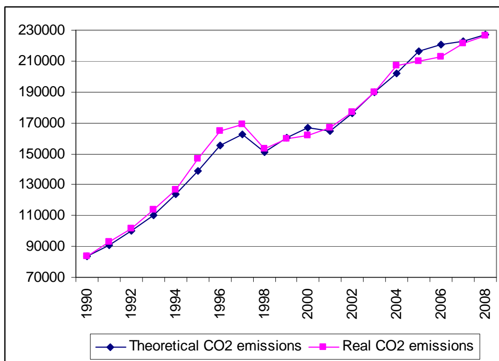
Figure 22 - Theoretical and real CO 2 emissions for the overall economy, 1990-2008
