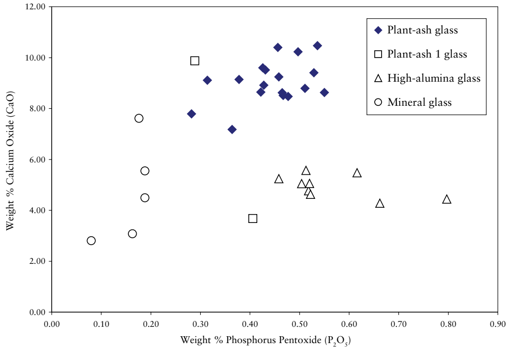
FIG. 6. Relative levels of phosphorus pentoxide ( P_2O_5 ) and calcium oxide (CaO) in bangles from Tell Abu Sarbut and Khirbat Faris.
