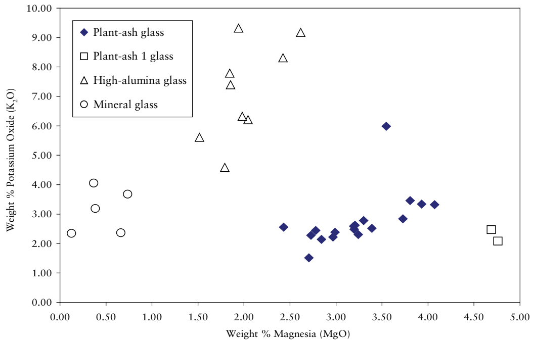
FIG. 5. Relative levels of magnesia ( MgO ) and potassium oxide ( K_2O ) in bangles from Tell Abu Sarbut and Khirbat Faris.
