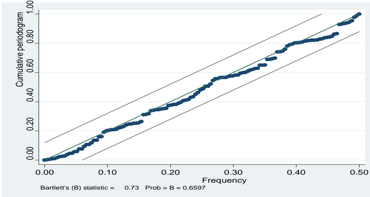
Figure.6: Cumulative Periodogram White-Noise Test for \hat{\varepsilon}_t .
