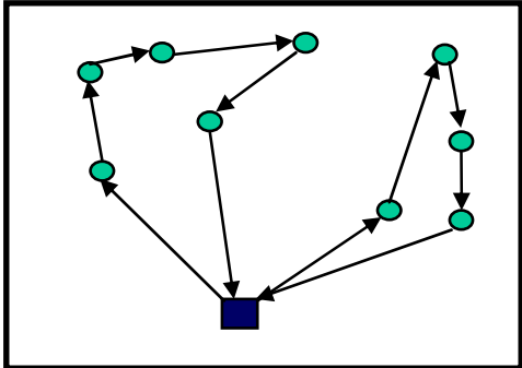
Single Echelon Approach (Dantzig and Ramser, 1959)
