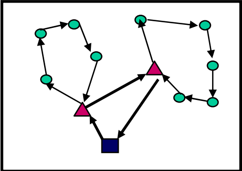
Two-Echelon Approach (Gonzalez-Feliu, 2008)
