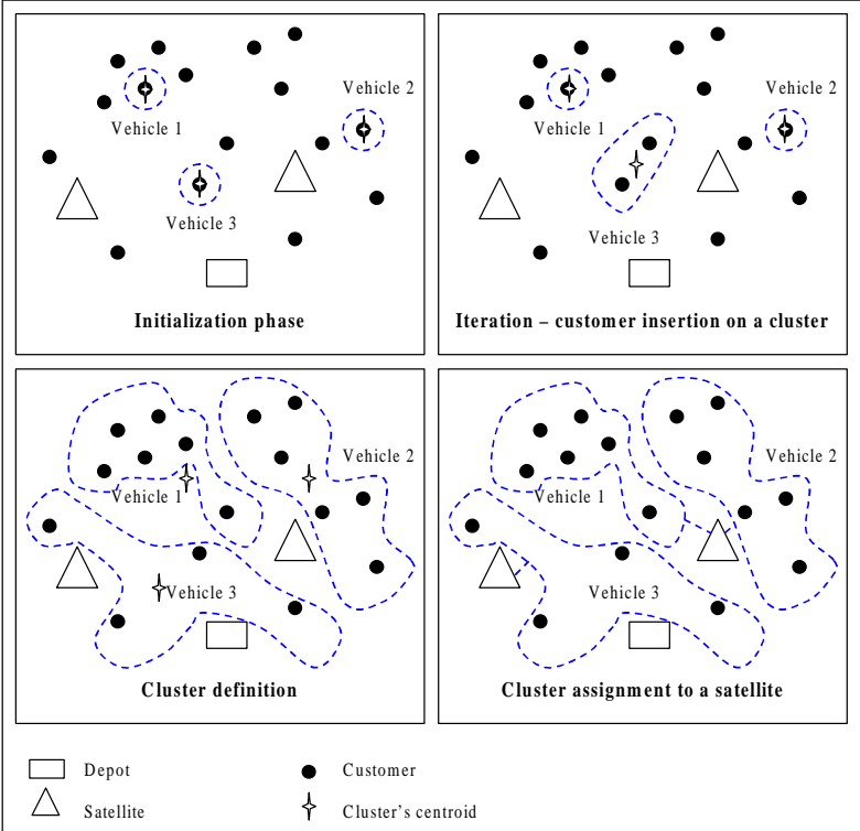
Figure 3 – Schema of the Semi-Greedy Algorithm for the Second-Echelon Routes
