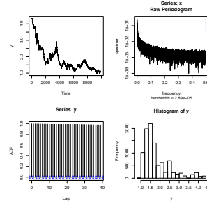
Figure 16: Trajectory, ACF, spectrum and histogram of Switzerland/U.S. exchange rate.
