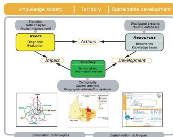
Diagram 2: CATALYSE method
