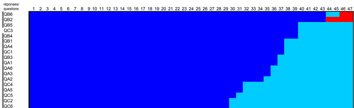
Fig 3. Synthesis of Delphi 5
