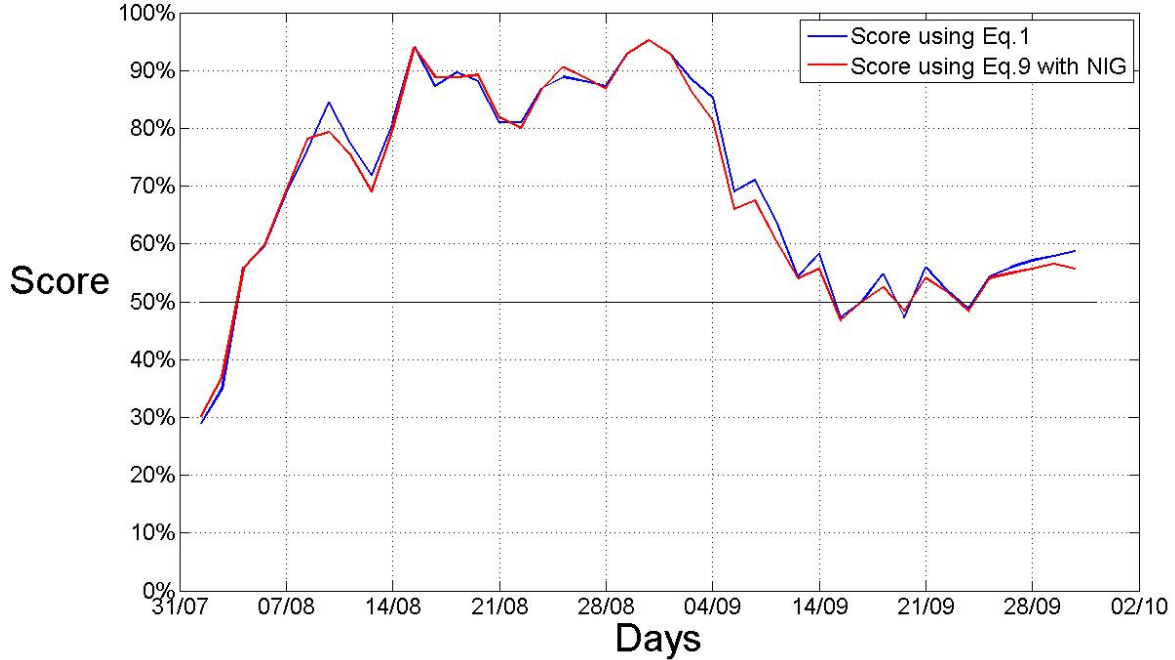
Figure 6: Observed score S_t and approximated score \bar{S}_t of the invested LSEW portfolio defined in Table 3 from the 31/07/2009 at the closing and over the 42 following days. The score S_t is obtained by enumeration over all the LSEW portfolios and thus is the real score of the invested portfolio. \bar{S}_t is the approximated score of the invested portfolio obtained by fitting with a NIG distribution and assuming (A_0) and (A_1) .
