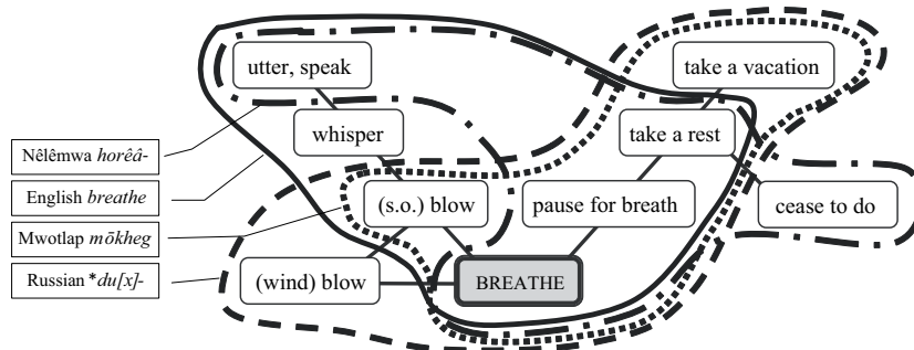
Figure 4 – Some isolectic sets around the notion {BREATHE}
