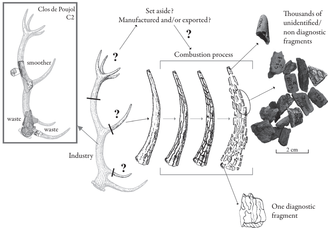
Figure 17: Explanatory chart of the discarding and burning patterns about Cervid antlers from Level C2 (Early Montclusian) at Clos de Poujol (photo A. Bridault, CAD E. David).
