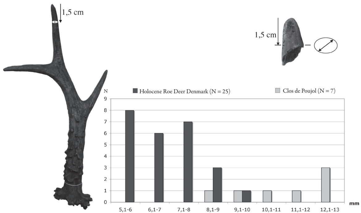
Figure 13: Distribution of the largest diameters (measured at 1.5cm from the tip of tines) at Clos de Pujol, compared to those same measurements on Roe Deer antlers from Holocene sites archived at the Zoology Museum of Copenhagen. The illustration on the left belongs to a Roe Deer antler from Langesø Mose, Denmark (Photo A. Bridault, CAD E. David).
