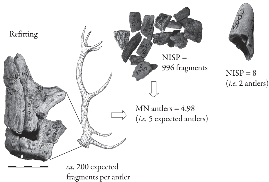
Figure 16: Assessment of the quantity of antlers present in unit C2 and their preservation state (complete or incomplete). Comparison between an assessment of the number of antlers (based on the number of antler tips inventoried in that same unit) and an assessment of the expected number of complete antlers (based on the number of fragments). Antler drawing from Billamboz 1977, fig. 3. Scale in centimetre (photo S. Oboukhoff & A. Bridault, CAD E. David).
