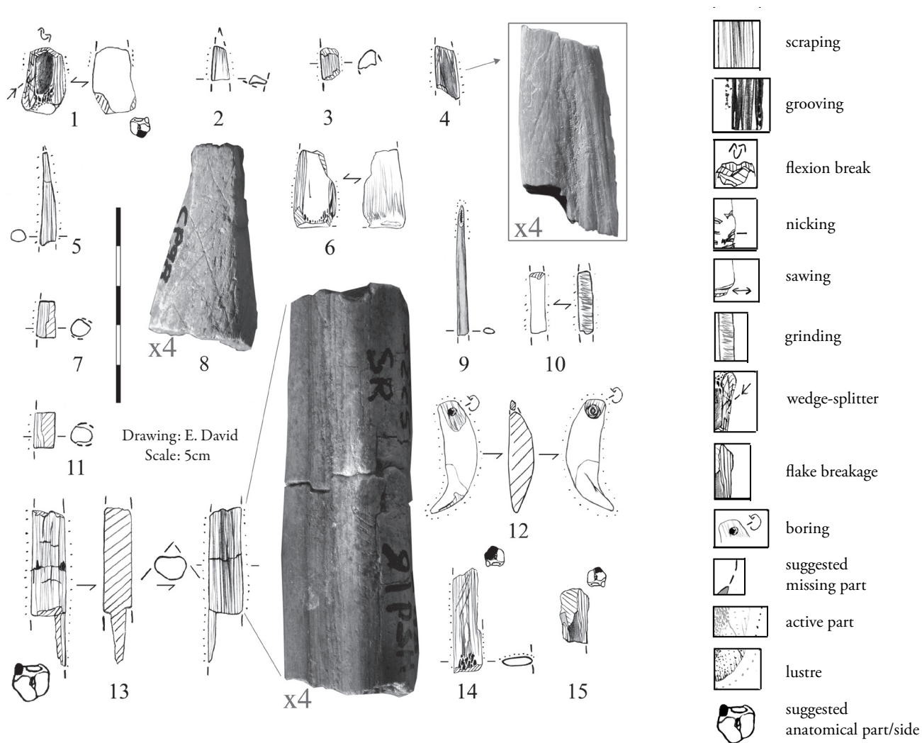
Figure 4: Osseous (bone/tooth) industry from Clos de Poujol (see Table 3). In bold, artefacts attributed in the field to the Middle Mesolithic: 1- Awl-like tool fragment (Red Deer metapodial); 2- Awl-like tool tip fragment (Roe Deer metapodial); 3- Straight point-like tool fragment (large mammal bone); 4- Awl-like tool fragment, active part (Roe Deer metapodial); 5- Straight point fragment (mammal bone); 6- Pointed tool base fragment (Roe Deer metapodial); 7- Straight point shaft fragment (Red Deer metapodial); 8- Engraved (?), unidentified fragment (mammal bone); 9- Thin needle-like fragment, active part (Badger fibula); 10- Pointed tool shaft fragment (mammal bone); 11- Straight point shaft fragment (Red Deer metapodial); 12- Pendant-type perforated item (Dog or Badger canine); 13- Straight point shaft fragment (Red Deer metapodial); 14- Unidentified tool fragment (base) (Roe Deer metapodial); 15- Débitage waste fragment (Roe Deer metapodial) (CAD E. David).
