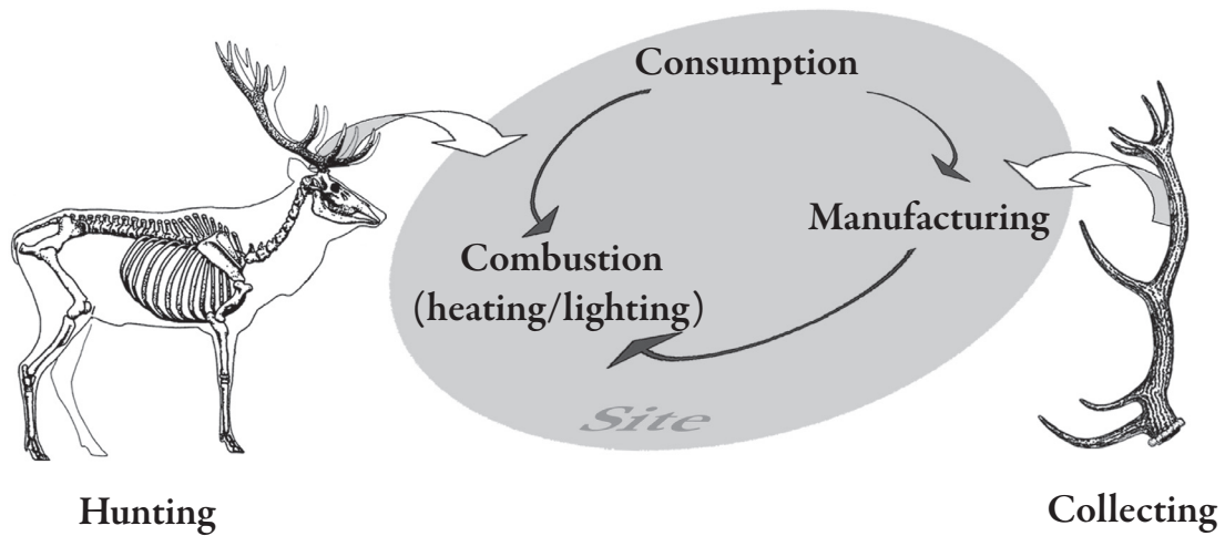
Figure 1: Theoretical model of Red Deer exploitation in the Mesolithic at Clos de Poujol. Deer skeleton, from Bonnet & Klein, 1991, p.36 (CAD E. David).
