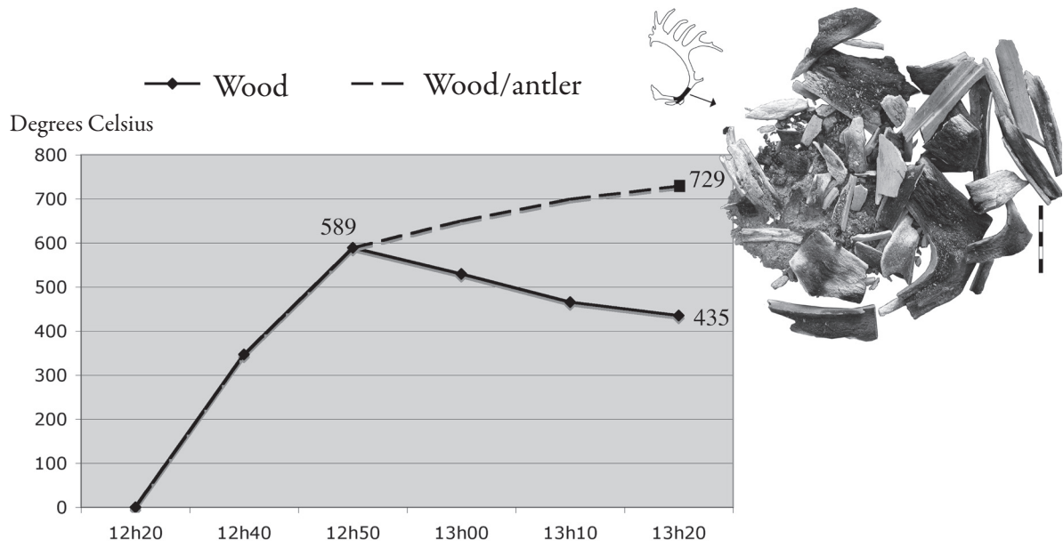
Figure 10: Physical appearance of burnt Reindeer antler. Temperatures reached in a reference hearth using wood logs (Scale in cm) (photo A. Bridault, CAD E. David).
