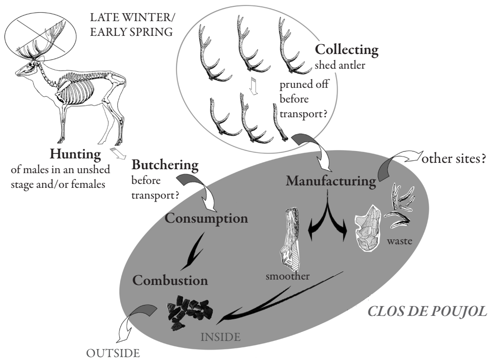
Figure 19: Restitution of the Red Deer exploitation process during the Sauveterrian at Clos de Poujol documenting two distinct types of procurement (collect of shed antler and animal hunting) carried out at the end of winter and/or the beginning of spring (CAD E. David).
