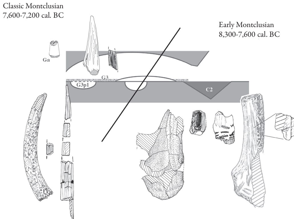
Figure 9: Stratigraphic distribution of the osseous industry (total of 14 items) attributed to the Sauveterrian at Clos de Poujol. Beside an unidentified fragment (not drawn here), four artefacts correspond to the initial phase (Early Montclusian) and nine others to the following phase (Classic Montclusian) (CAD E. David).
