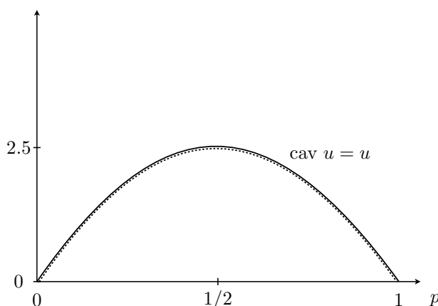
Note. Plot of the functions u(p) (dotted lines) and \text{cav } u(p) (plain lines) against p \in [0, 1] for the NR-game in Figure 1.
