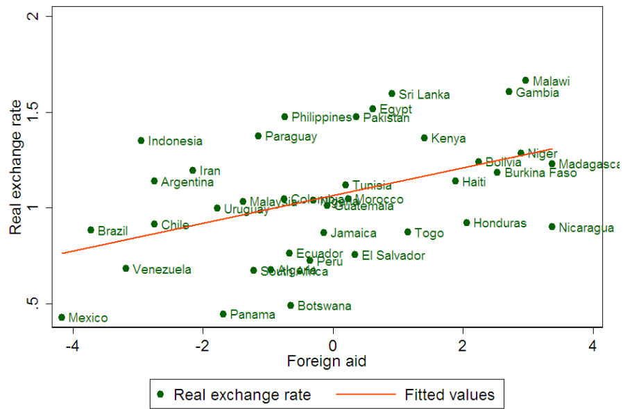
Figure 3: Unconditional correlation - RER and Foreign Aid in 2004.
