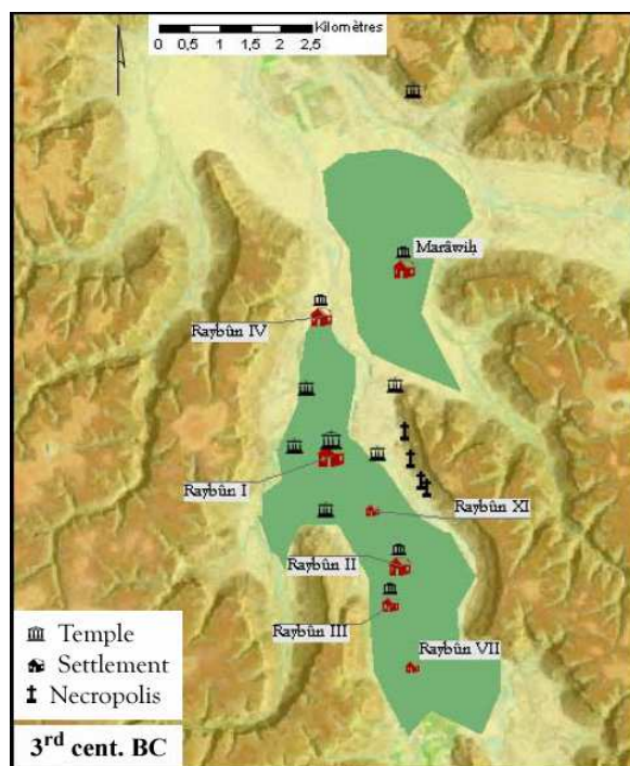
Figure 10 : Sketch-map of the Raybūn area (3rd cent. BC)
