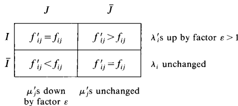
Diagram 2. Changes when neither M nor N labelled. a' = a .
