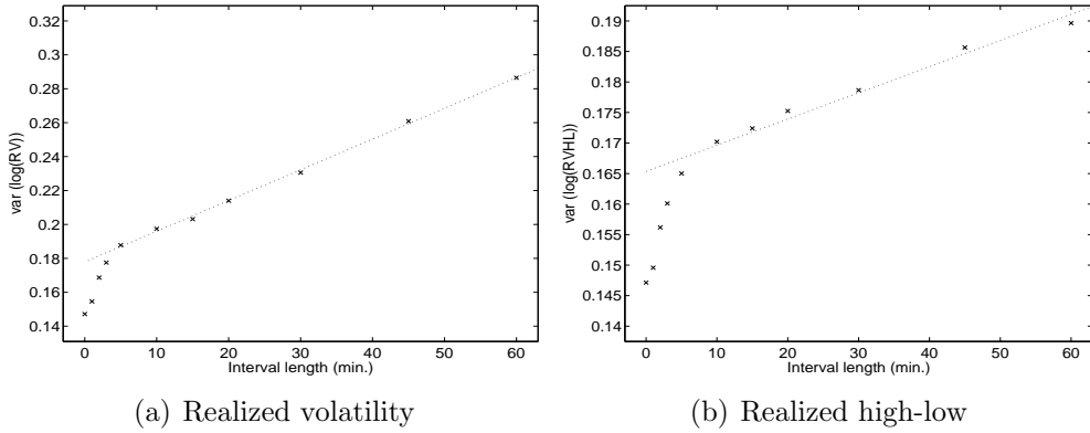
Figure 3: Plots of the sample variance of the log of a proxy with \Delta t ranging from zero to 60 minutes (zero is tick per tick). (a) Realized volatility. (b) Realized high-low.
