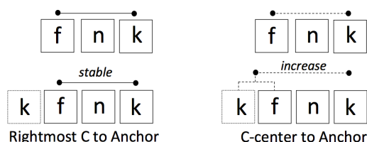
Figure 2. Predictions for right-edge stability in Tashlhiyt syllables.
