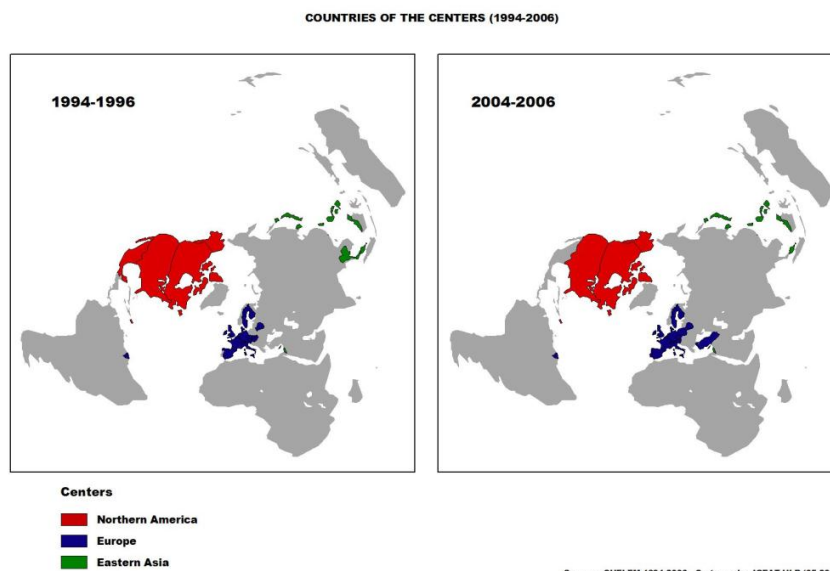
Figure 23: Clustering of core's countries (Steps E and F) - 1994-96 - All products - Export
