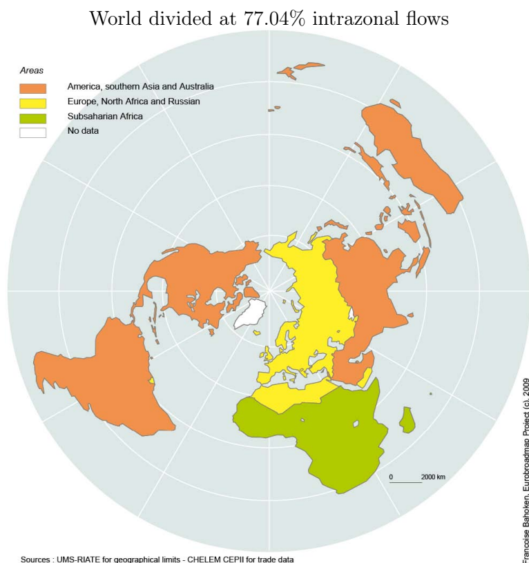
Figure 6: Intramax clustering on Chelem's international trade flows (1994-96) - 1
