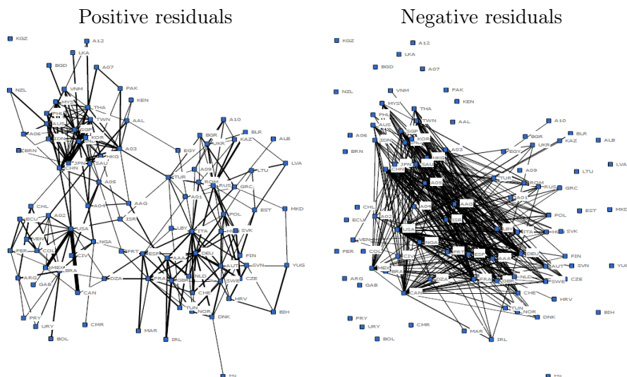
Figure 10: Graph of most significant residuals for Trade 2004-06
