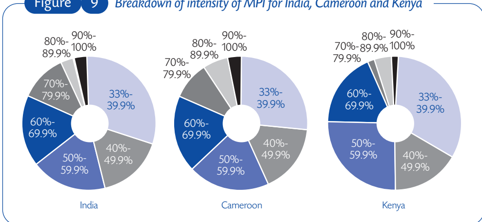
Figure 9 Breakdown of intensity of MPI for India, Cameroon and Kenya
