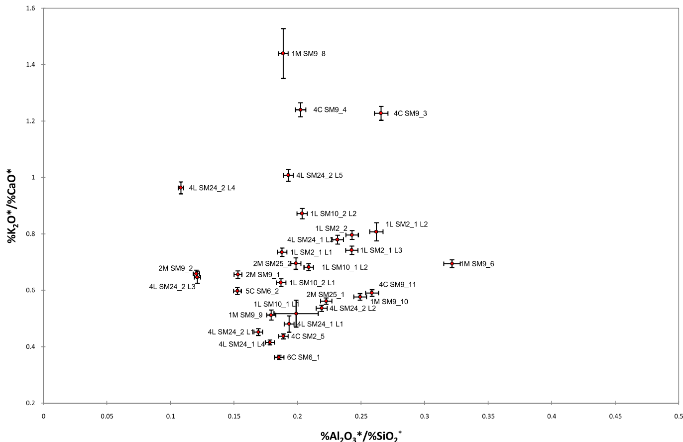
Fig. 13. NRC ratios in the slag inclusions: Al_2O_3^*/SiO_2^* versus K_2O^*/CaO^* .
