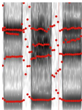
Figure 7: Spectrogram corresponding to the central part of [i], spoken in isolation (left), in the uvular context [ʁiʁ] (mid), and to the vowel /e/ (right). Spoken by the author.
