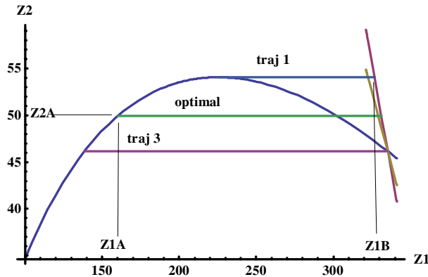
Figure 5: Possible solutions
