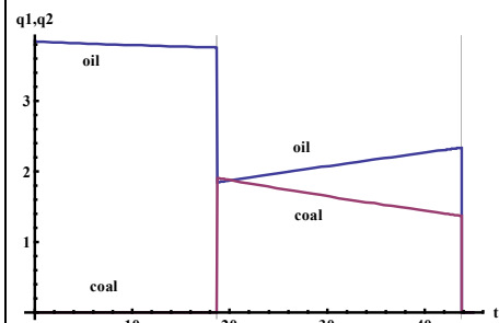
Figure 6 Extraction rates (time)
