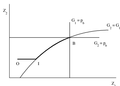
Figure 2: Extraction path 1
