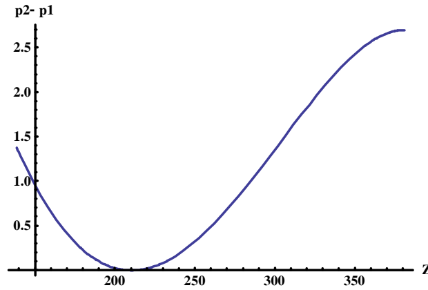
Figure 9: The solution
