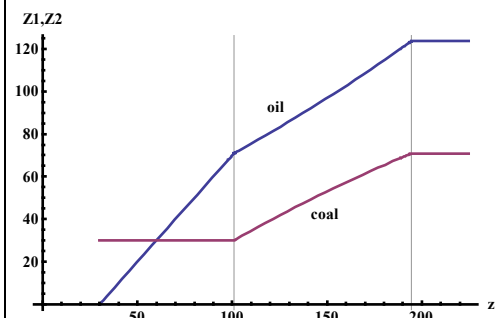
Figure 4 Extraction paths
