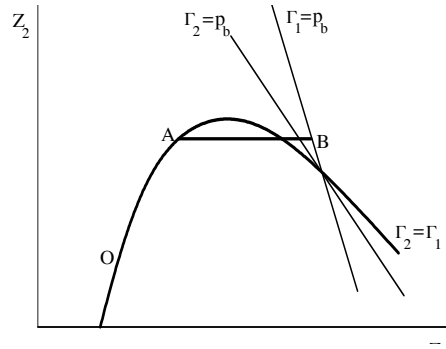
Figure 4: Forsaking resource 2
