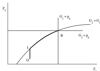
Figure 2: Extraction path 1
