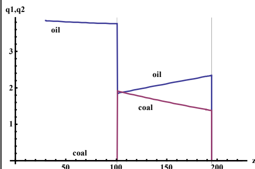
Figure 5 Extraction rates
