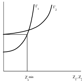
Figure 1: Extraction costs
