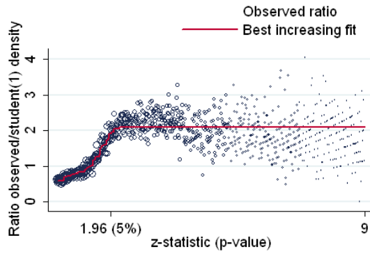
(c) Best increasing non-parametric fit for the ratio of densities output/Student input.
