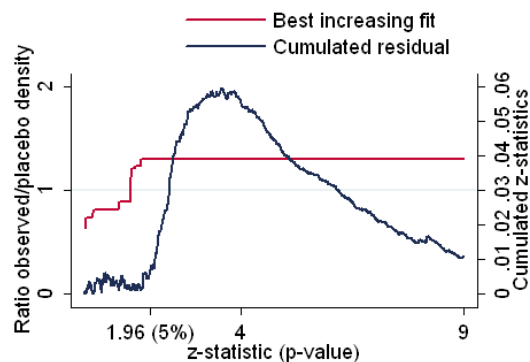
(b) Cumulated residual (WDI placebo input).
