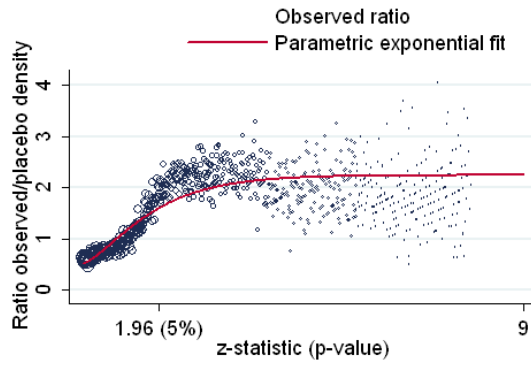
(c) Best increasing parametric fit for the ratio of densities output/Student input.
