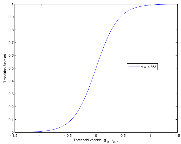
Figure 1: Estimated transition function ( c=0 ) for the OCRS specification
