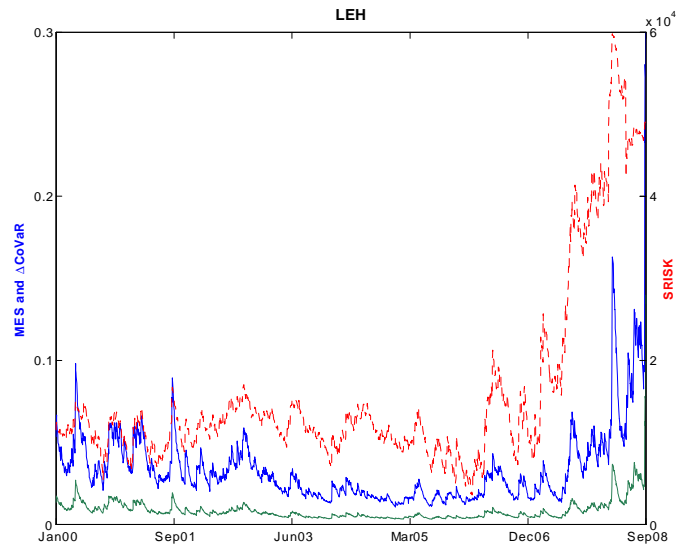
Figure 1: Time Series Evolution of Systemic Risk Measures: The figure displays the MES (middle solid line, left axis), the \Delta\text{CoVaR} (bottom solid line, left axis) and the SRISK (top dashed line, right axis) of Lehman Brothers (LEH). The estimation period is from 01/03/2000 to 09/17/2008.
