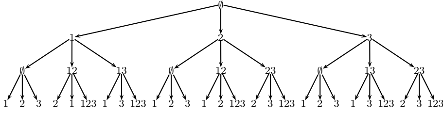
Fig. 3 Set of scenarios \mathfrak{S}(\mathbf{U}^{\mathbf{M},\infty}, 3)
