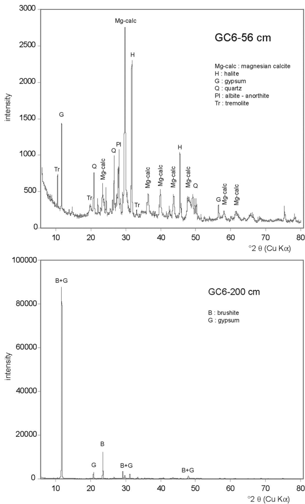
Figure 7. Mineralogical composition of a carbonate mud layer (GC6, 56 cm) and an evaporitic layer (GC6, 200 cm). Quartz, albite-anorthite, and tremolite derive from the granodiritic substrate, while magnesian calcite, gypsum and brushite are authigenic minerals. Halite is thought to have precipitated during sample drying the water column, in connection with pond lowstands (Figure 10B). High photosynthesis activity favoured by shallow water promotes saturation with respect to calcite and carbonate precipitation (Kelts and Hsü, 1978), and also strongly influences the
