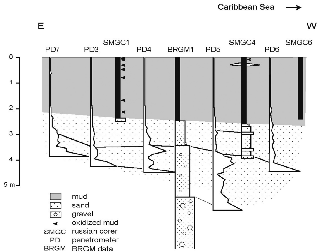
Figure 3. Schematic cross section of the lake infilling. PD, penetrometer; BRGM, cores made by the Bureau de Recherche Géologique et Minière, France; SMGC, cores used for this study (GC1, GC4 and GC6)
