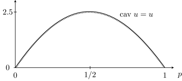
Note. Plot of the functions u(p) (dotted lines) and \text{cav } u(p) (plain lines) against p \in [0, 1] for the NR game in Figure 1.
