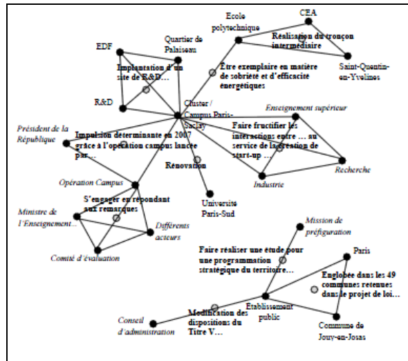
Figure 3: Simplicial Complex of our Google™ query.
