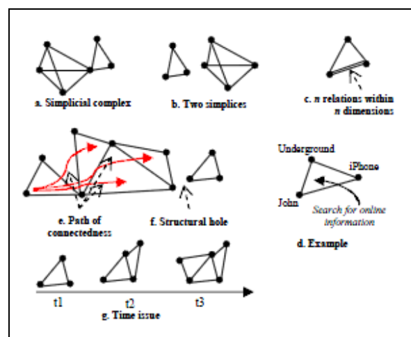
Figure 5: Main notions of the simplicial.
