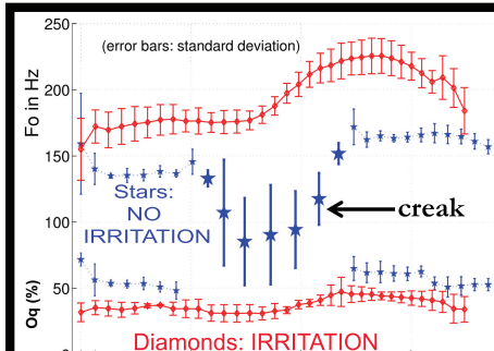
Fig. 4. Average curves of F0 and Oq over 6 tokens of /da3/, speaker M6
