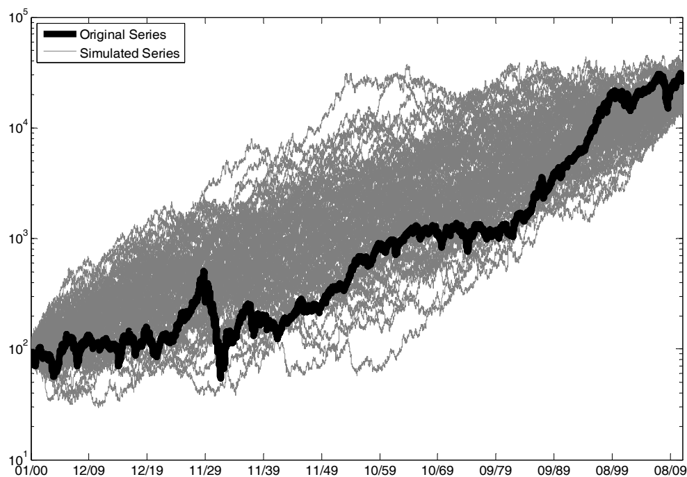
An Illustration of some Artificial DJIA-based Series
