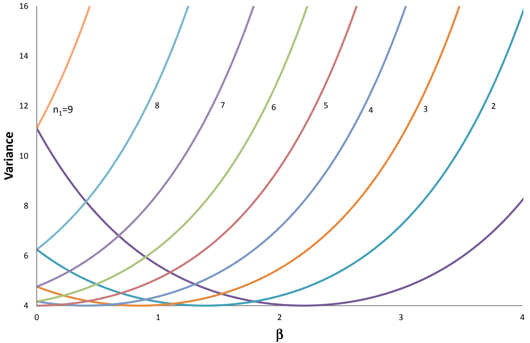
Fig. 1: Variance with respect to \beta and n_1 for the MNL ( n=10 )
