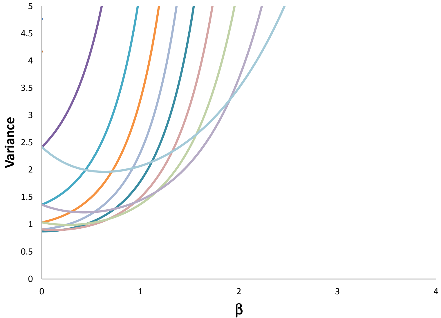
Fig. 2: Variance with respect to \beta and n_1 Worst choice observed ( n=10 )
