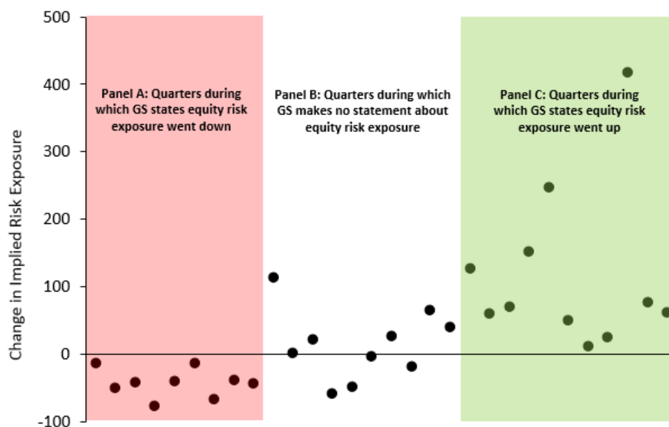
Figure 2: Empirical Performance of the FIRE Methodology
