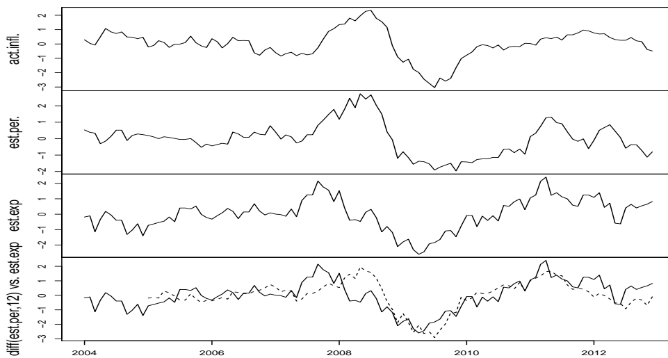
Figure 3: Raw estimates of perceptions and expectations; differentiated perceptions vs. expectations - Jan 2004 to Dec 2012
