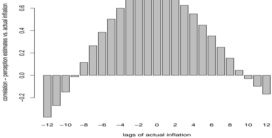
Figure 4: Correlation - Perceptions vs. actual Inflation - Jan 2004 to Dec 2012
