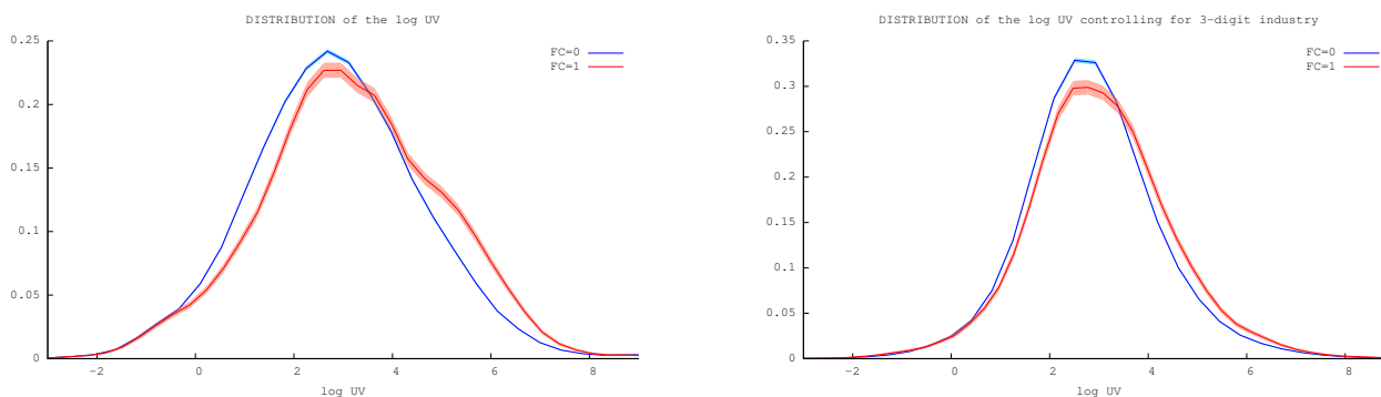
Figure 1: EMPIRICAL DENSITY OF (log) UNIT VALUES.
