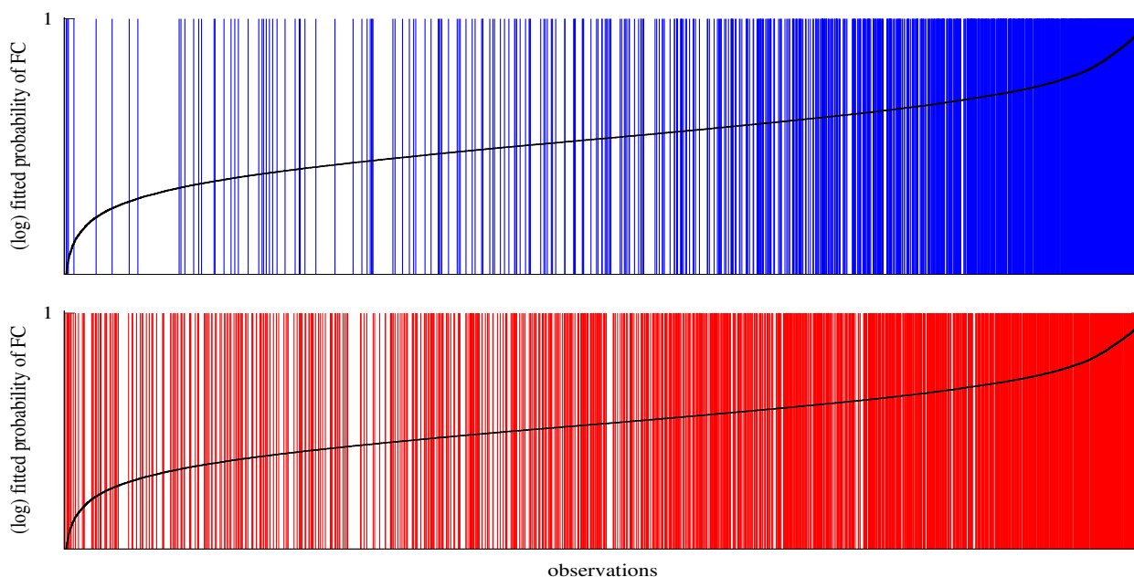
Figure A4: PROBIT SEPARATION PLOT
