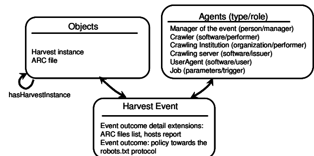
Figure 3. Aligning web archiving concepts with PREMIS
