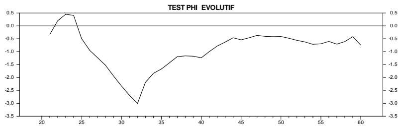
Figure 3.11.3 – Harvey and Collier Phi-test
