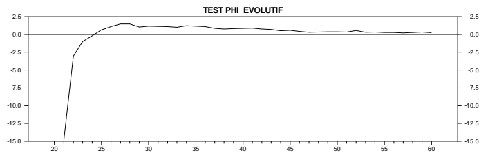
Figure 3.8.3 – Harvey and Collier Phi-test
