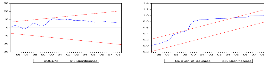
Figure 3.8.2 – CUSUM and CUSUM squared test's results
