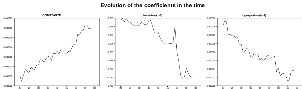
Figure 3.5.1 – Evolution of the coefficients
