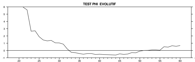
Figure 3.12.3 – Harvey and Collier Phi-test
