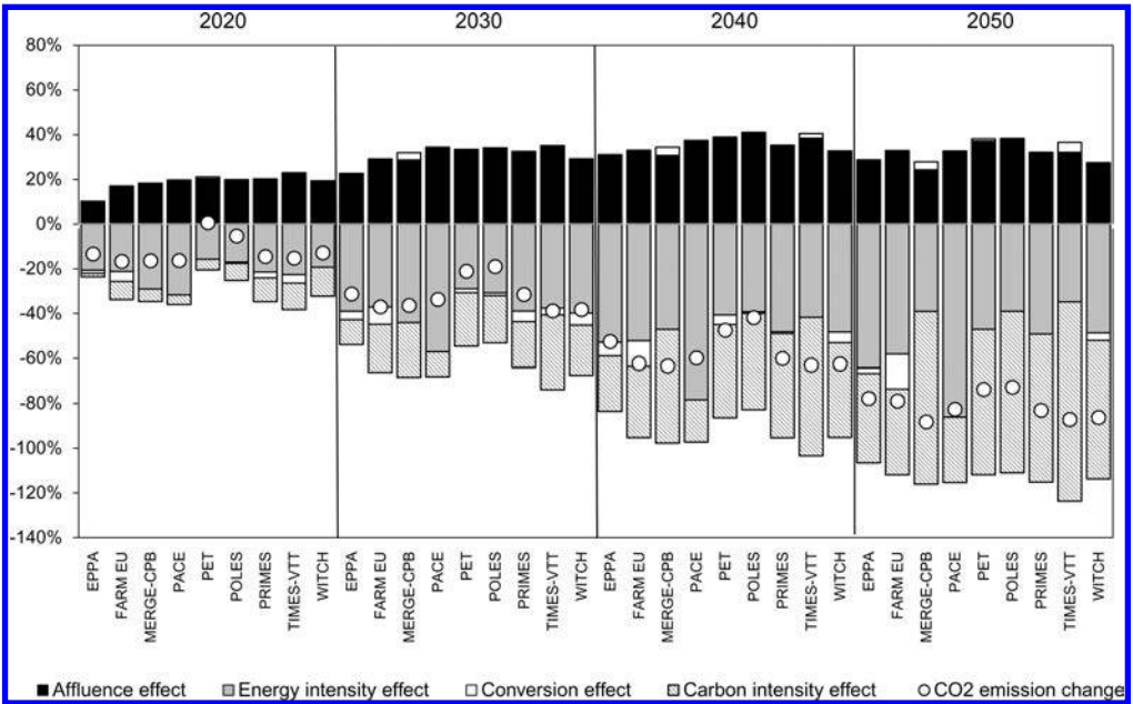
Figure 2. Results of decomposition over time for 80% DEF scenario for the EU-27. Base year = 2010. Results normalized to 2010 emissions. 7
