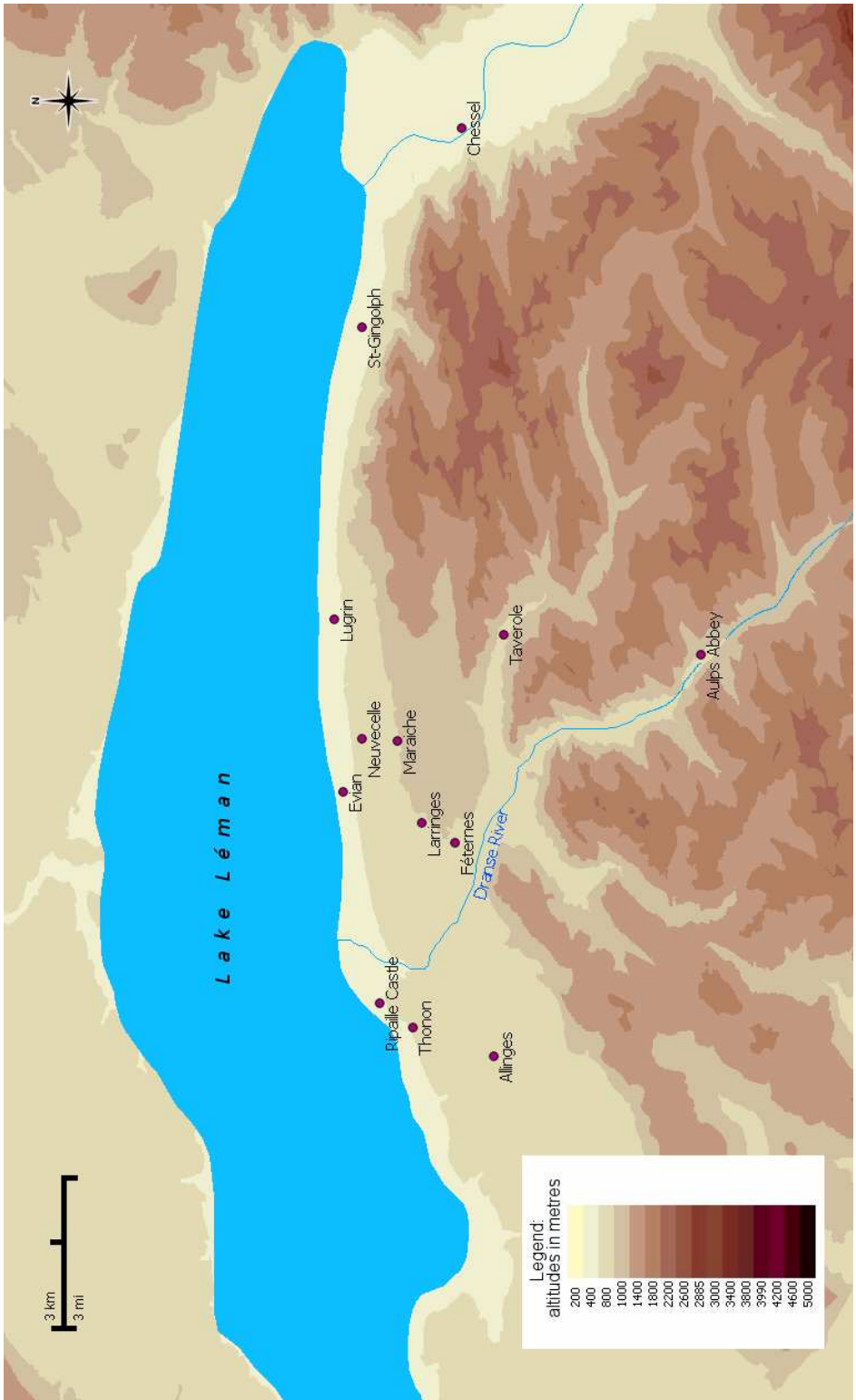
Figure 2. Map of the castellary of Evian-Féternes.
