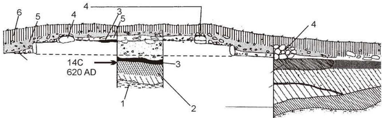
Fig. 4 : Stratigraphy of the Gavilan STR 5F-15 1- Limestone bedrock 2- Paleosoil 3- Stucco level 4- House wall 5- Collapse level 6- Present day soil
