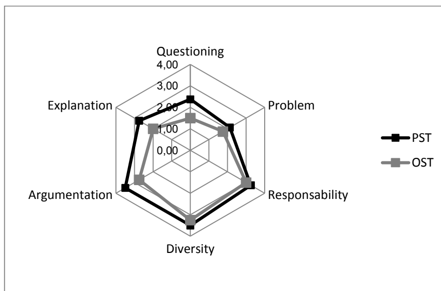
Figure 1: Locating teachers’ strategies on IBST 6 dimension model
