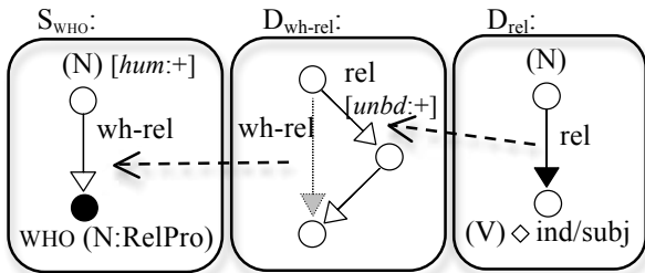
Figure 13. Rules for wh-relatives
