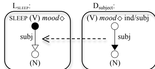
Figure 5. Lexical vs. dependency rules 7
