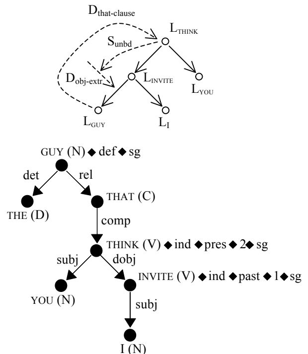
Figure 18. Derivation structure and derived tree for (4)
