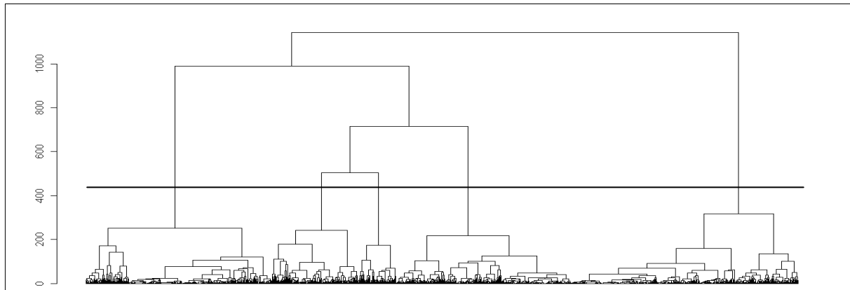
Figure 4a – Dendrogramme de la classification
